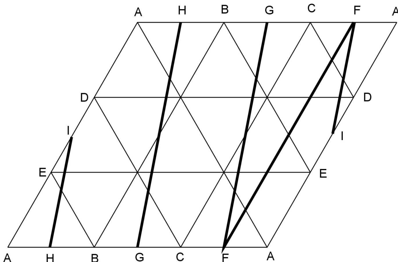
Figure 6. The s-torus.
