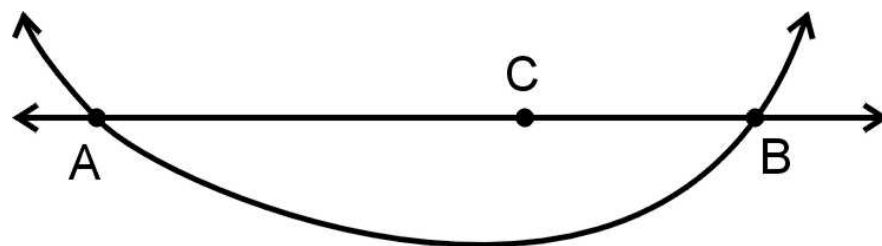
Figure 15. The point C lies only partially between A and B.
