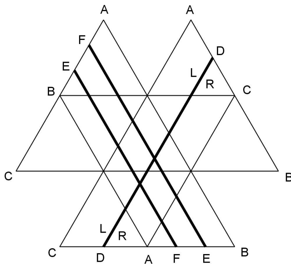
Figure 5. The s-projective plane.
